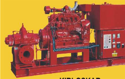
KIRLOSKAR DIESEL ENGINE FIRE FIGHTING PUMPSET
