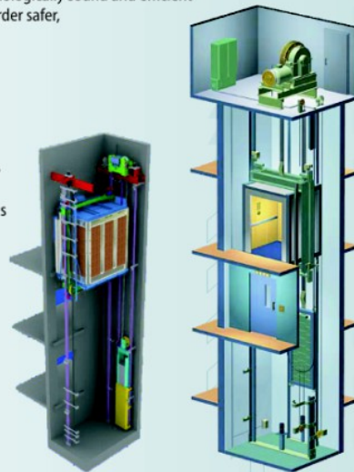
MRL Elevator
