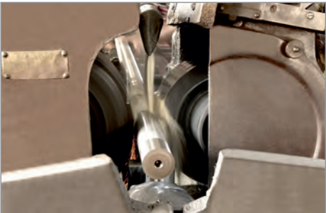
Centreless Grinding
