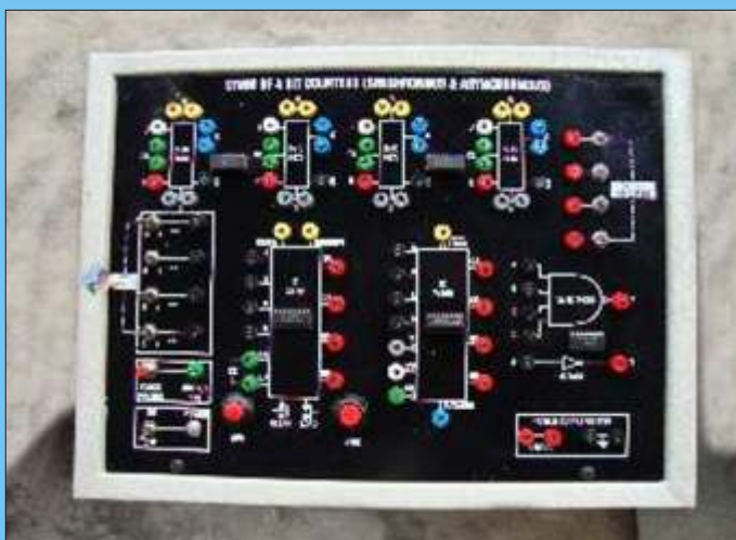
4 Bit Counter
