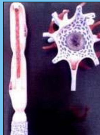
Neuron
