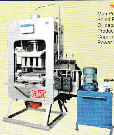
Semi Auto Brick Machine
