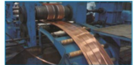
Slitting Line
