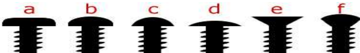
(a) pan, (b) button, (c) round, (d) truss, (e) flat (countersunk), (f) oval
