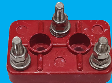
EF KH PRIME 1 3 STUD TYPE
