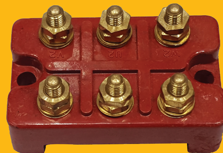
EF TEXMO 5 HP BK BRASS
